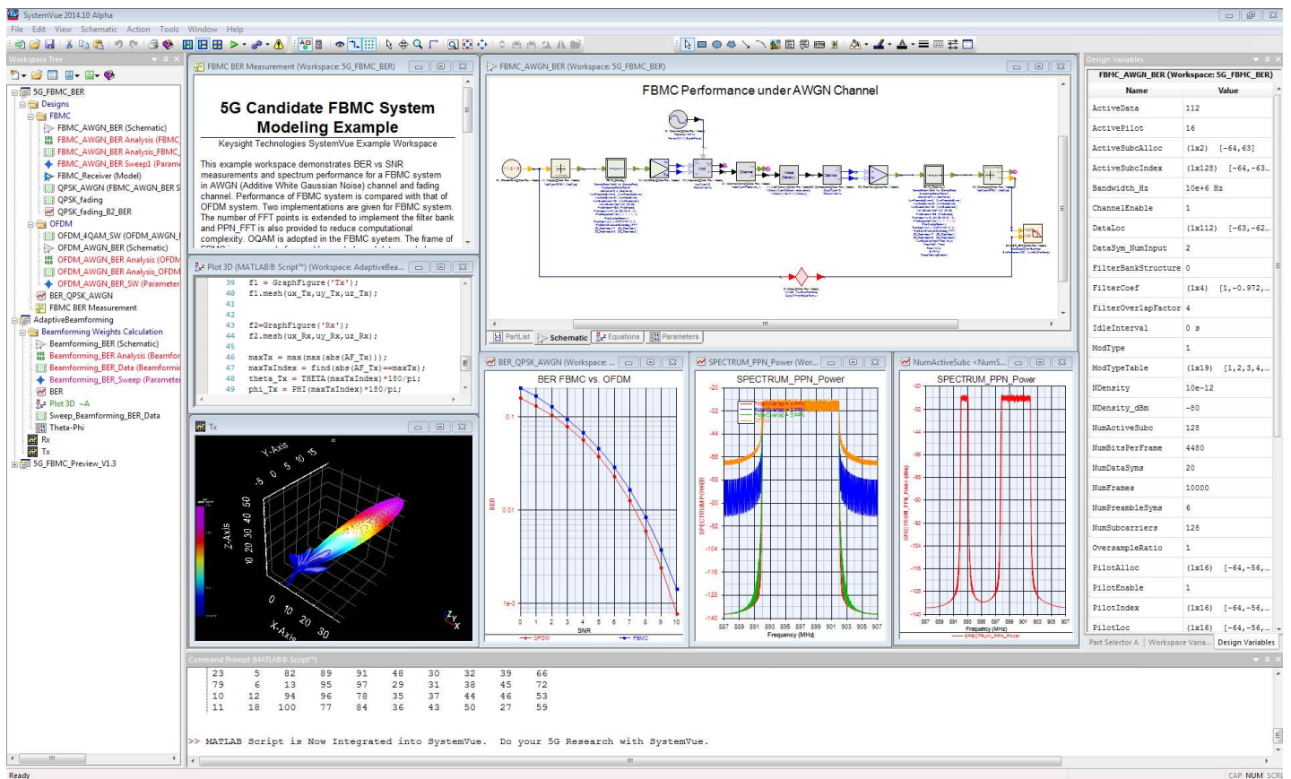
Figure 4. SystemVue's Baseband Exploration libraries build on top of verification libraries. They provide Keysight instrument-grade verification for algorithm developers in the earliest phases of a PHY design, so that ideas may be tested and proven right from the point of conception.
