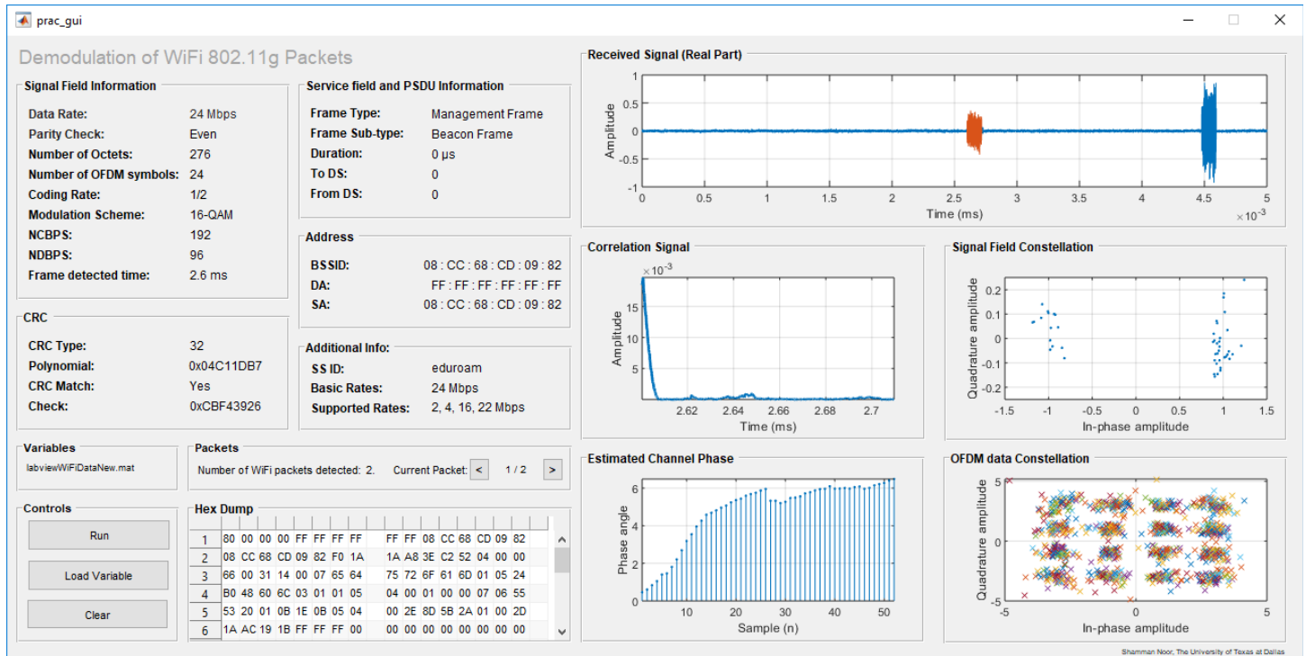
Fig. 3: SSID – ‘eduroam’, Subtype – Beacon, Variable: ‘labviewWiFiDataNew.mat’ – given, Packet number/ Total packets – 1/2 (2.6 ms)
